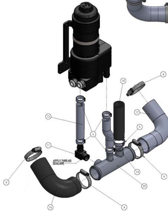
FINAL ASSEMBLY
