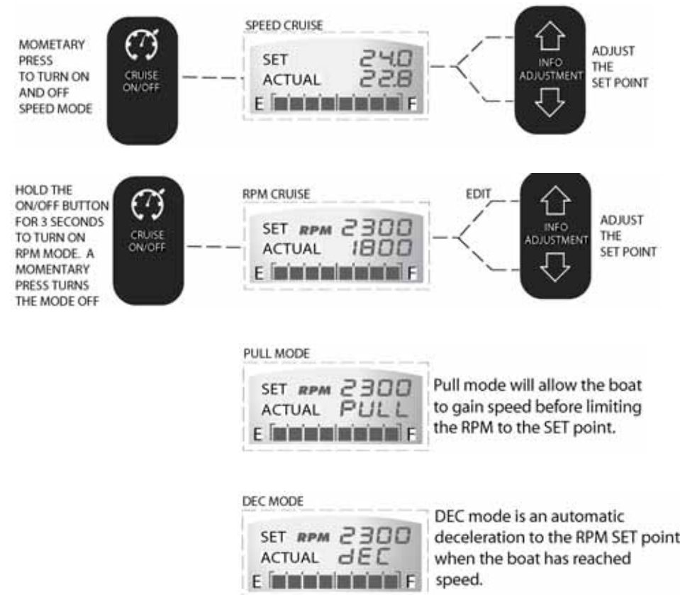
Figure 2-3. Speedometer
