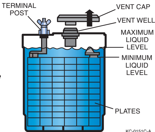
Figure 4-5. Battery Level
